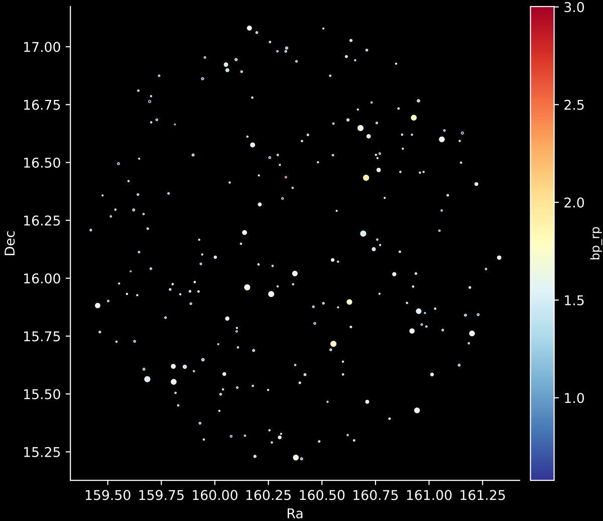
APOGEE DR17 Field: [175-27-O] Stars: 201
