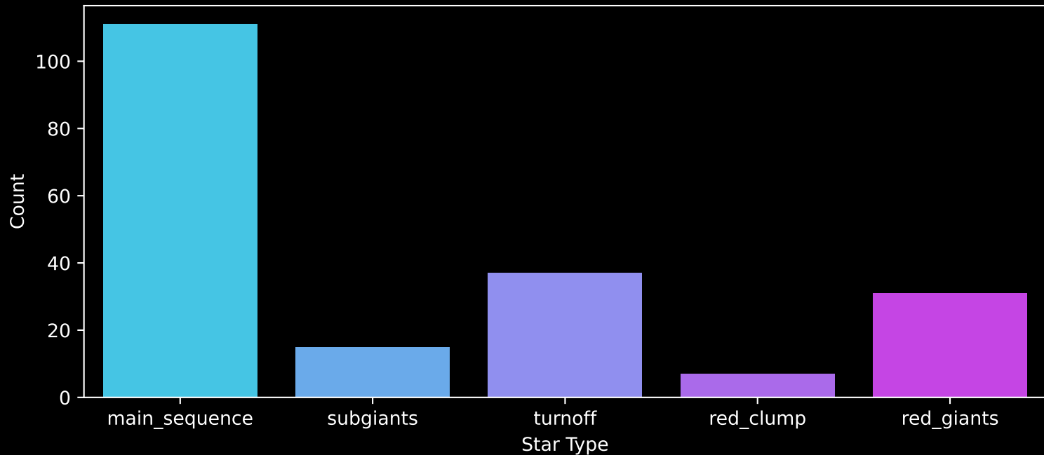
APOGEE DR17 Field: [175-27-O] Count plot of Star Type
