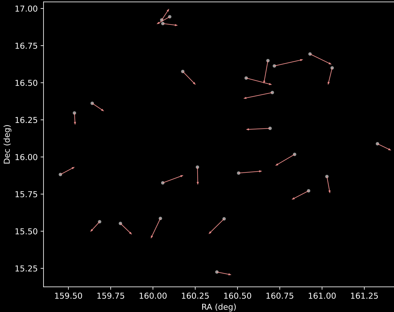
APOGEE DR17 Cluster 7 Proper Motion Vectors (n=26)
