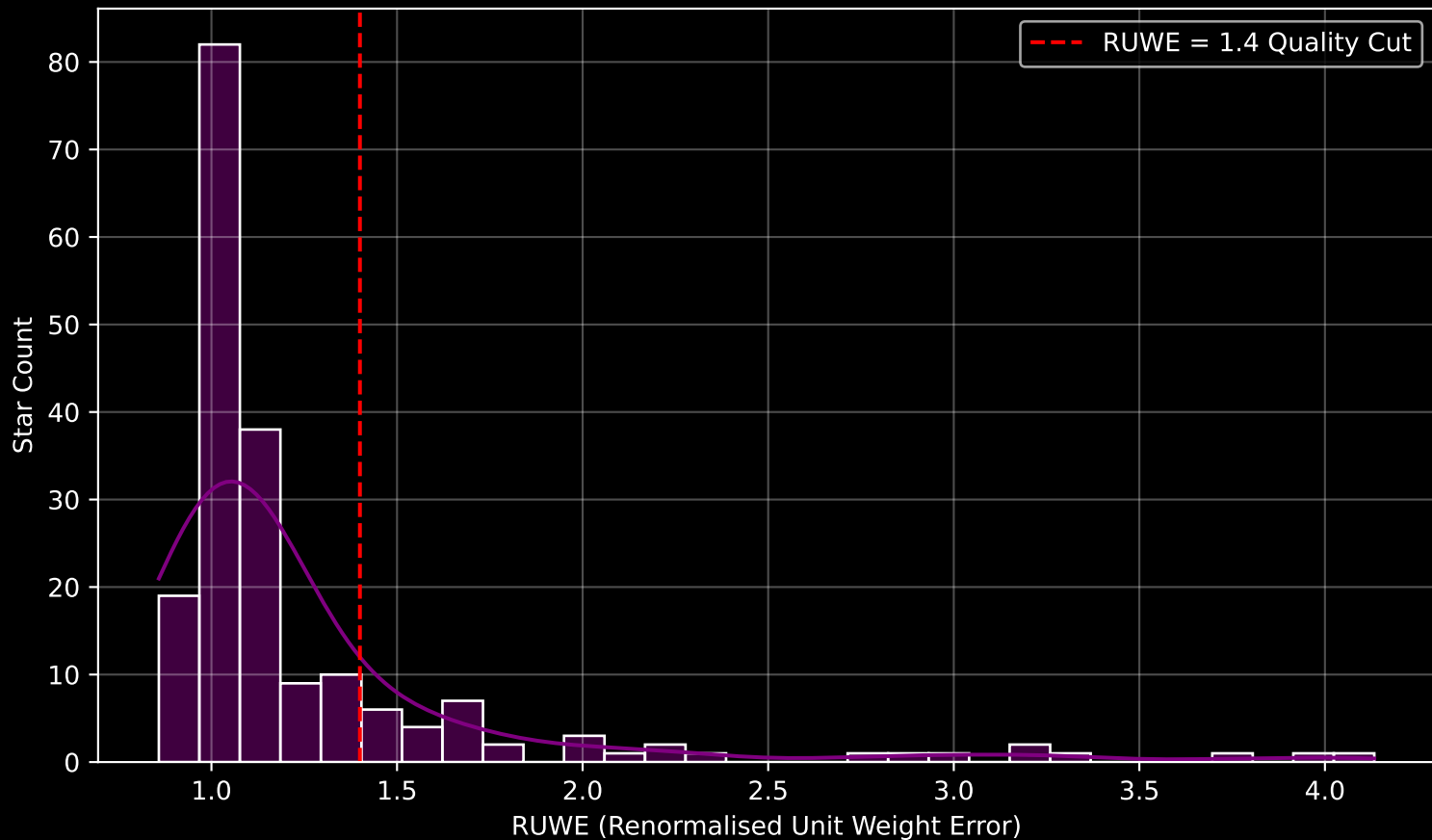
GAPOGEE DR17 Field [175-27-O] RUWE Distribution (n= 193)
