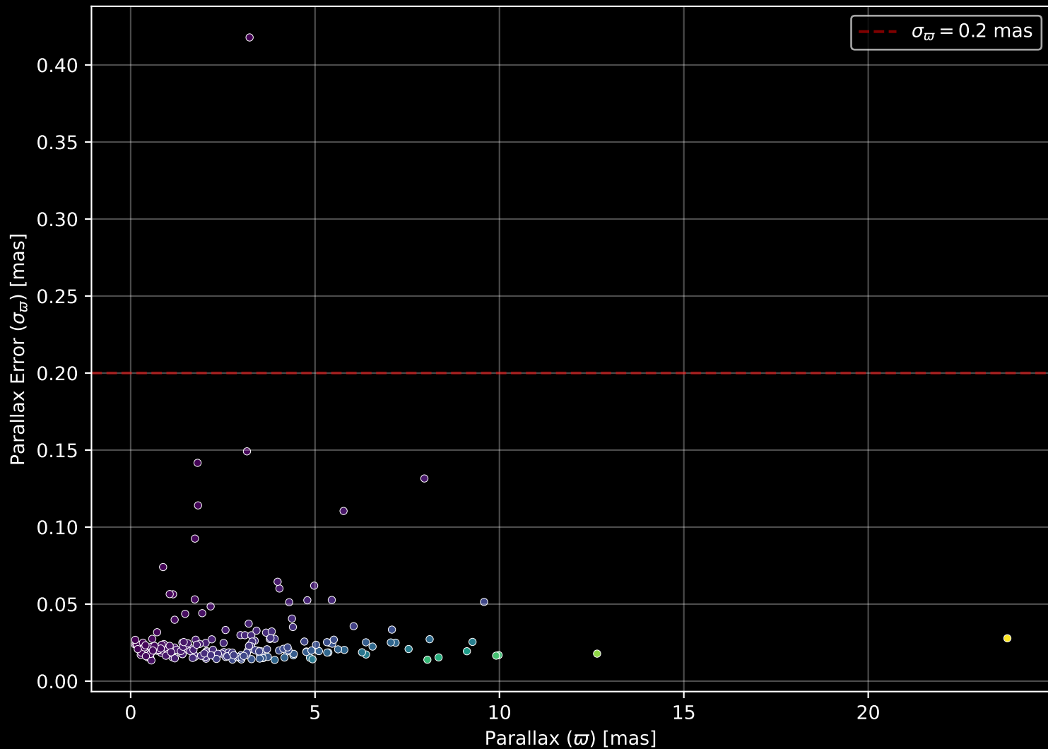
APOGEE DR17 Field: [175-27-O] Parallax Quality (n= 201)
