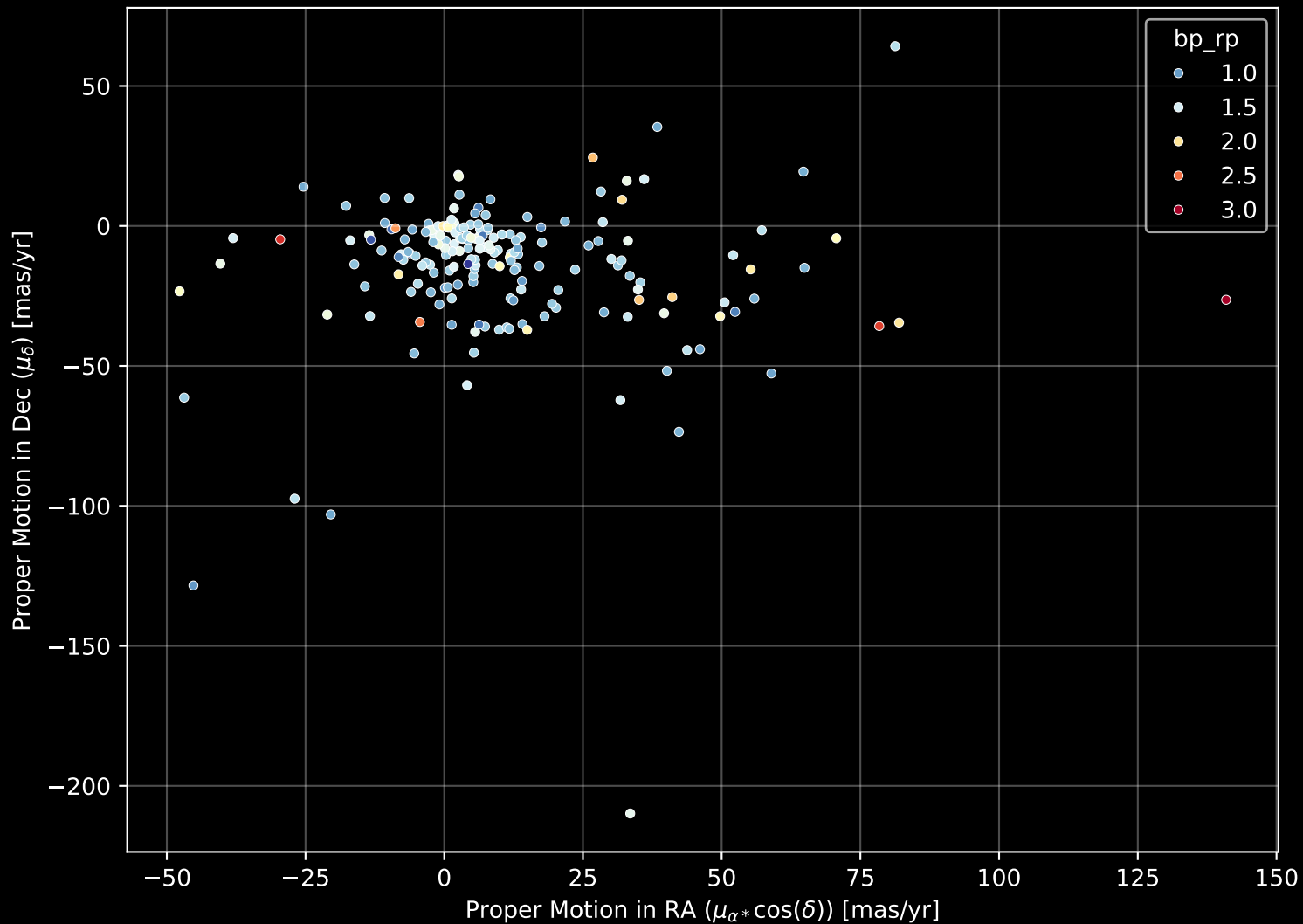
APOGEE DR17 Field: [175-27-O] Proper Motion Diagram (n= 201)
