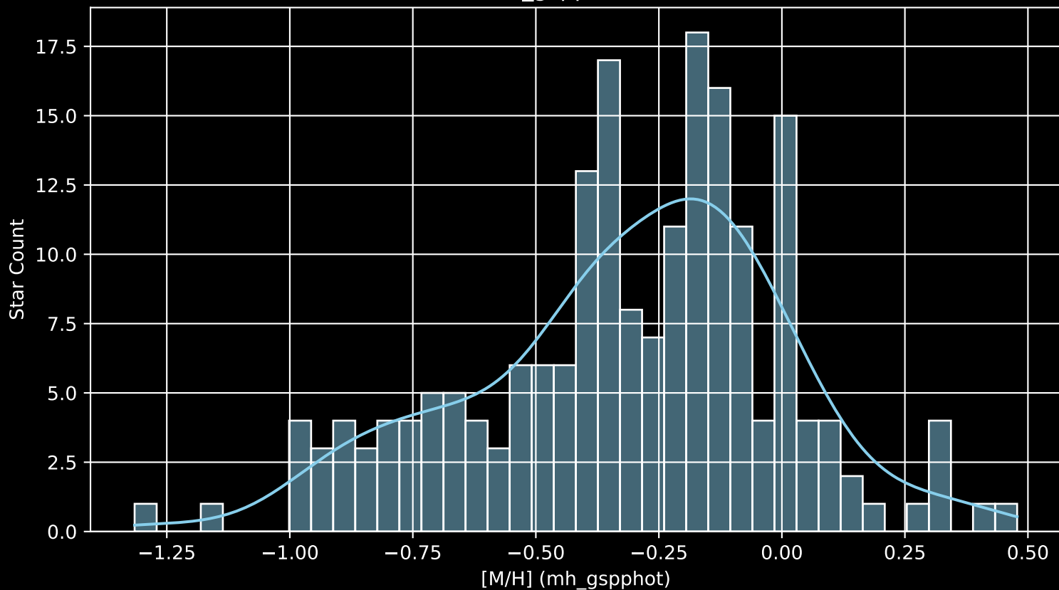
APOGEE DR17 Field: [175-27-O [M/H] (mh_gspphot) (n= 197)
