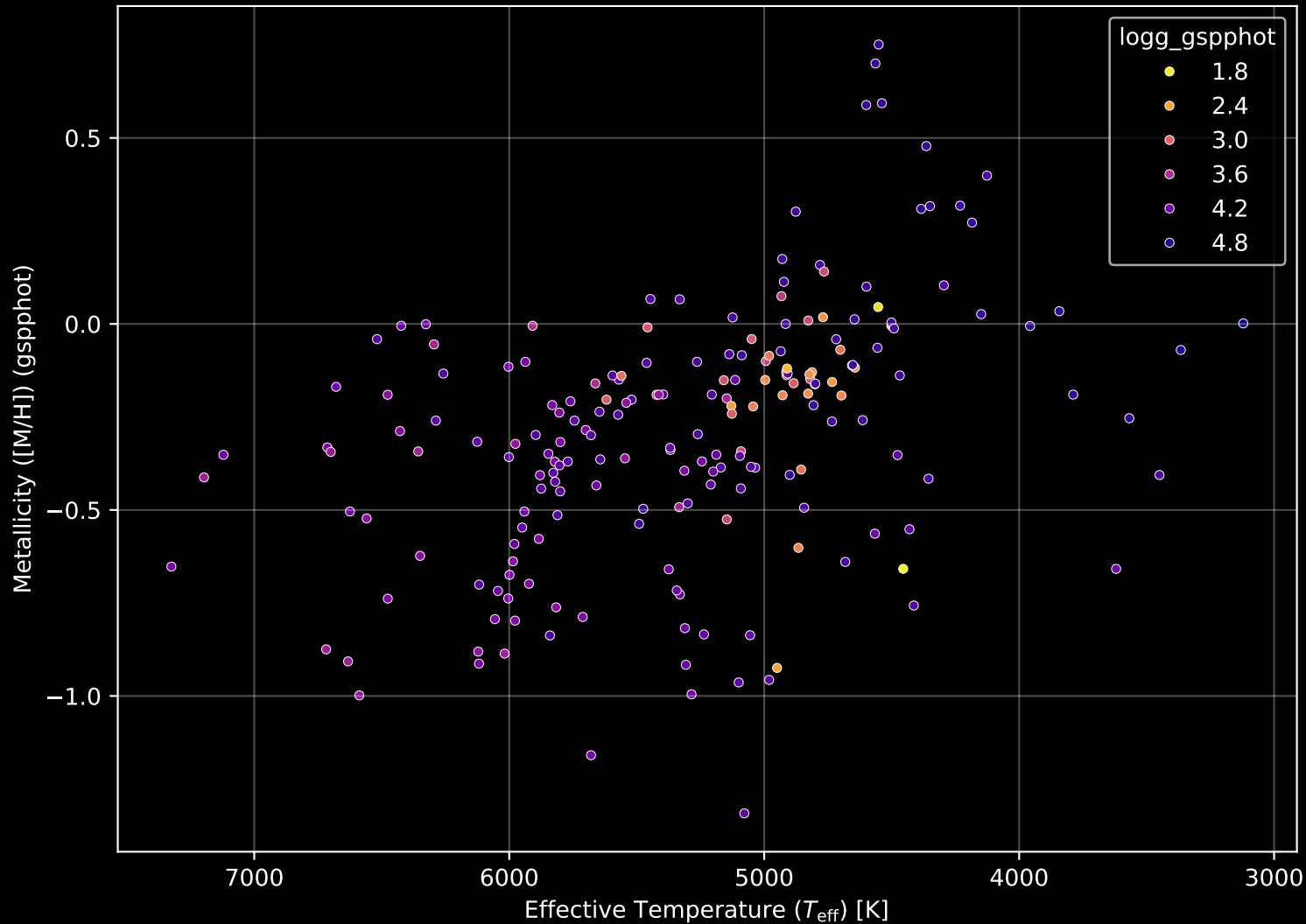
APOGEE DR17 Field: [175-27-O] Stellar Population Parameters (n= 201)
